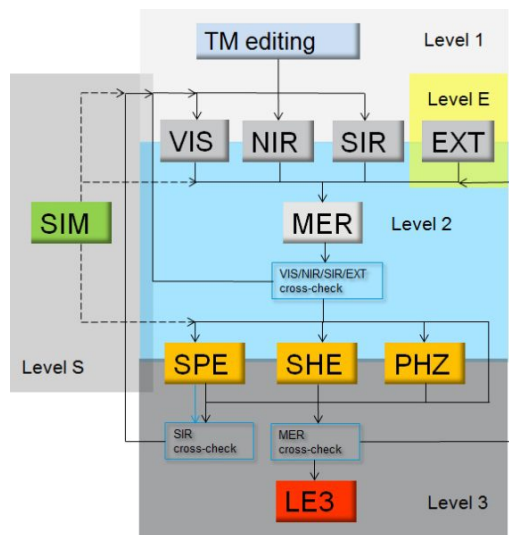
Figure 5: The SGS data processing organisation. Indicated are the different levels and the ten functions providing the data processing stages. The arrows indicate the flow of information between these stages. Level S is responsible for the provision of simulated data. Level E procures the external data from ground based surveys, most of these data are needed to complement the Euclid photometric measurements to derive the photometric redshifts of the WL galaxies down to the required accuracy of 5%..
