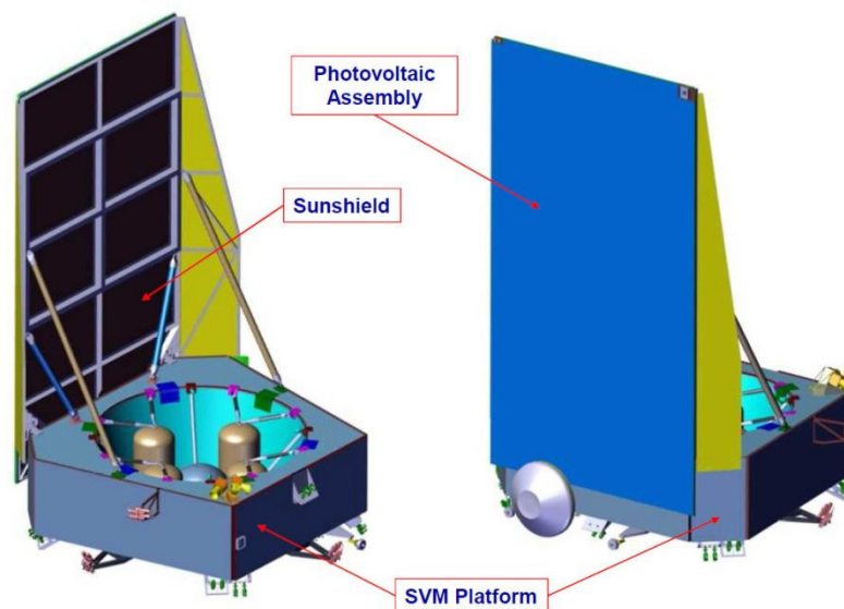
Figure 2: Views of the Euclid service module (SVM) with sunshield. Images of TAS-I (Turin)
