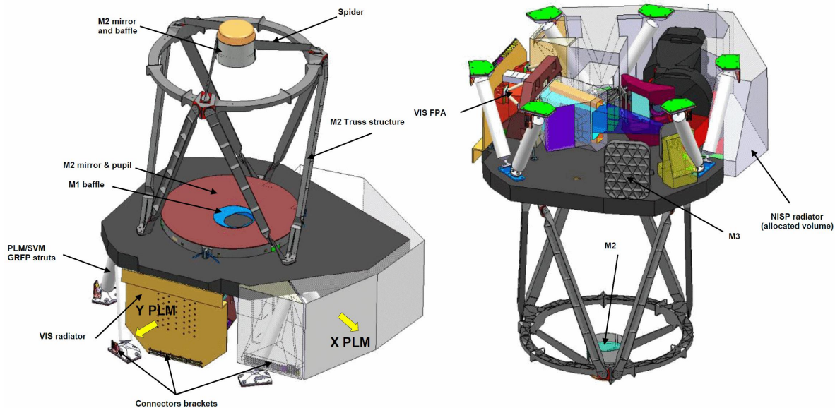
Figure 1: Top and bottom views of the PLM telescope with the VIS and NISP instruments. Image of Airbus Defense and Space, Toulouse.
