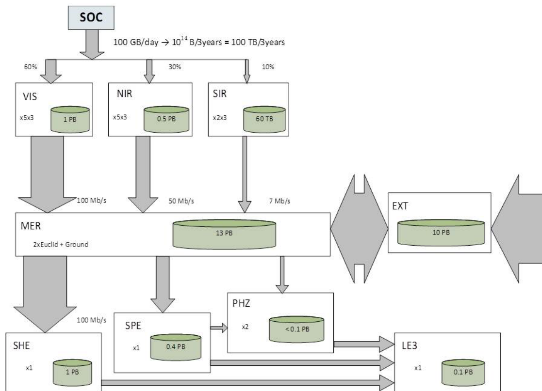
Figure 4. The data flow between the various processing functions of the SGS, and the related foreseen size. The size of the arrows representing the data flow are not to scale.
