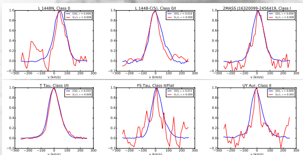
Figure: Comparison of the [OI] and o-H 2 O line profiles for sources whose [OI] profiles are better reproduced by multiple Gaussians. In the legends we show the measured \sigma of the Gaussian fits.
