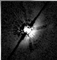
Scattered light imaging: dust Pinte+ (2008)
