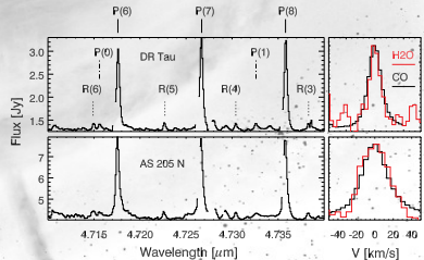
Near-IR spectroscopy: gas Salyk+ (2008)
