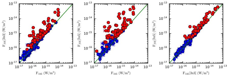
Figure: Extended emission tests for sources in the sample. Red dots identify sources showing extended emission in each of the tests used. The solid diagonal line depicts a one-to-one to help identifying extended emission.
