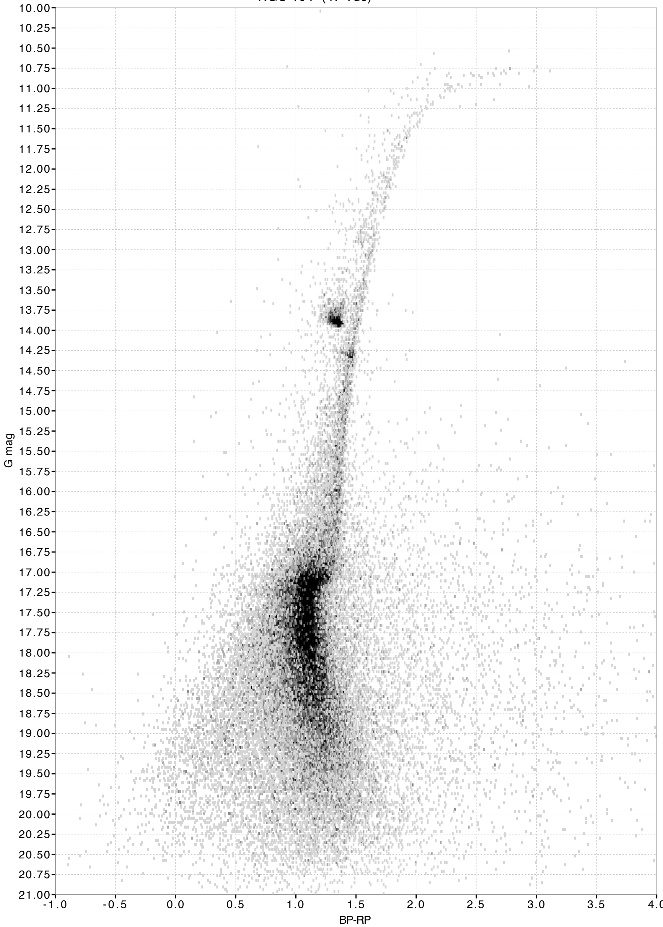
NGC 104 (47 Tuc)
