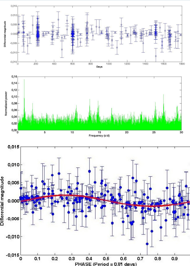
Example of time series analysis, with Gaia data (top), periodogram (middle) and folded light curve. A small amplitude sinusoidal variation can be fitted by a weighted period analysis method (here a least squares method) if the noise distribution is well known. In the periodogram the largest amplitude is found at frequency 1.23 cycle per day.
